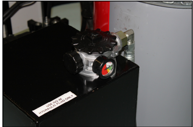
In tank hydraulic filter is quick and easy to change when required Indicator gauge shows when it is time for maintenance
