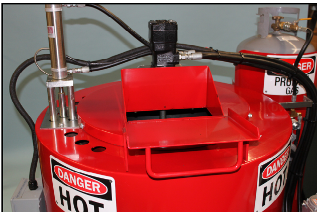
Large material fill port accepts all standard bituminous adhesives Hydraulic agitation system for durability
